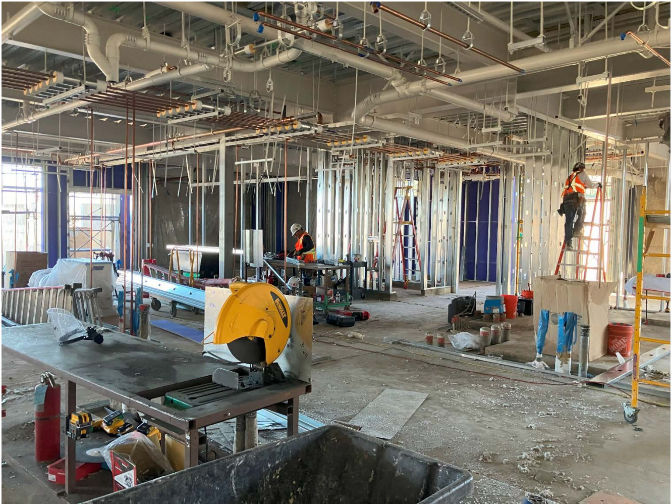
Interior Framing & Ceiling hung MEP's
