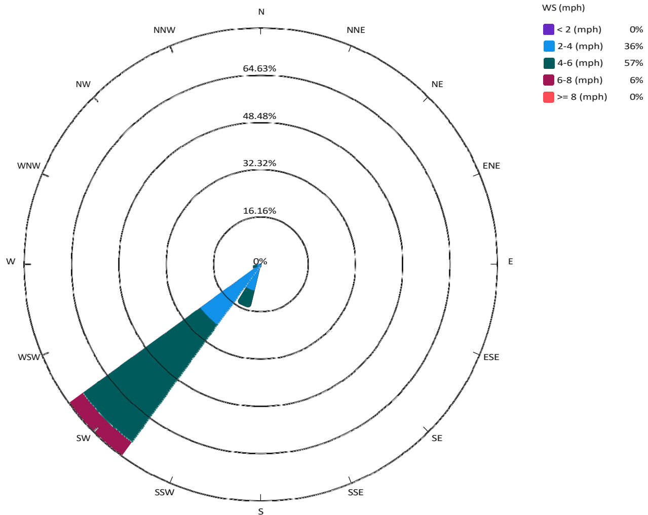
Wind rose (mph)
