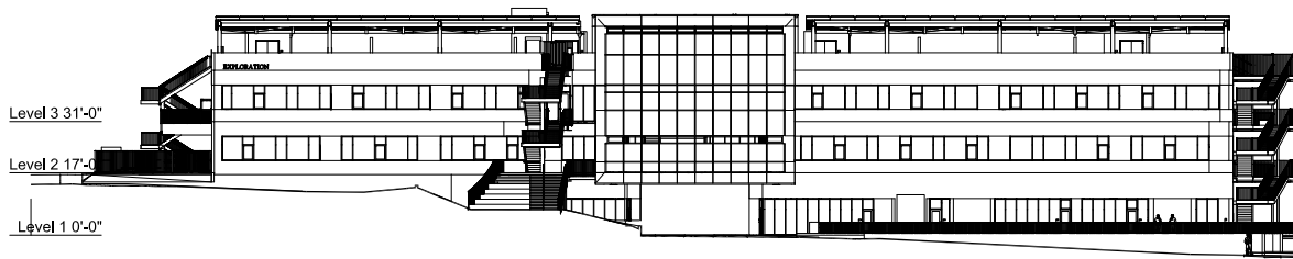
Exploration Building North Elevation
