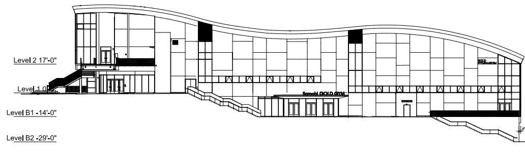
Gold Gym North Elevation
