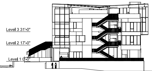
Exploration Building West Elevation
